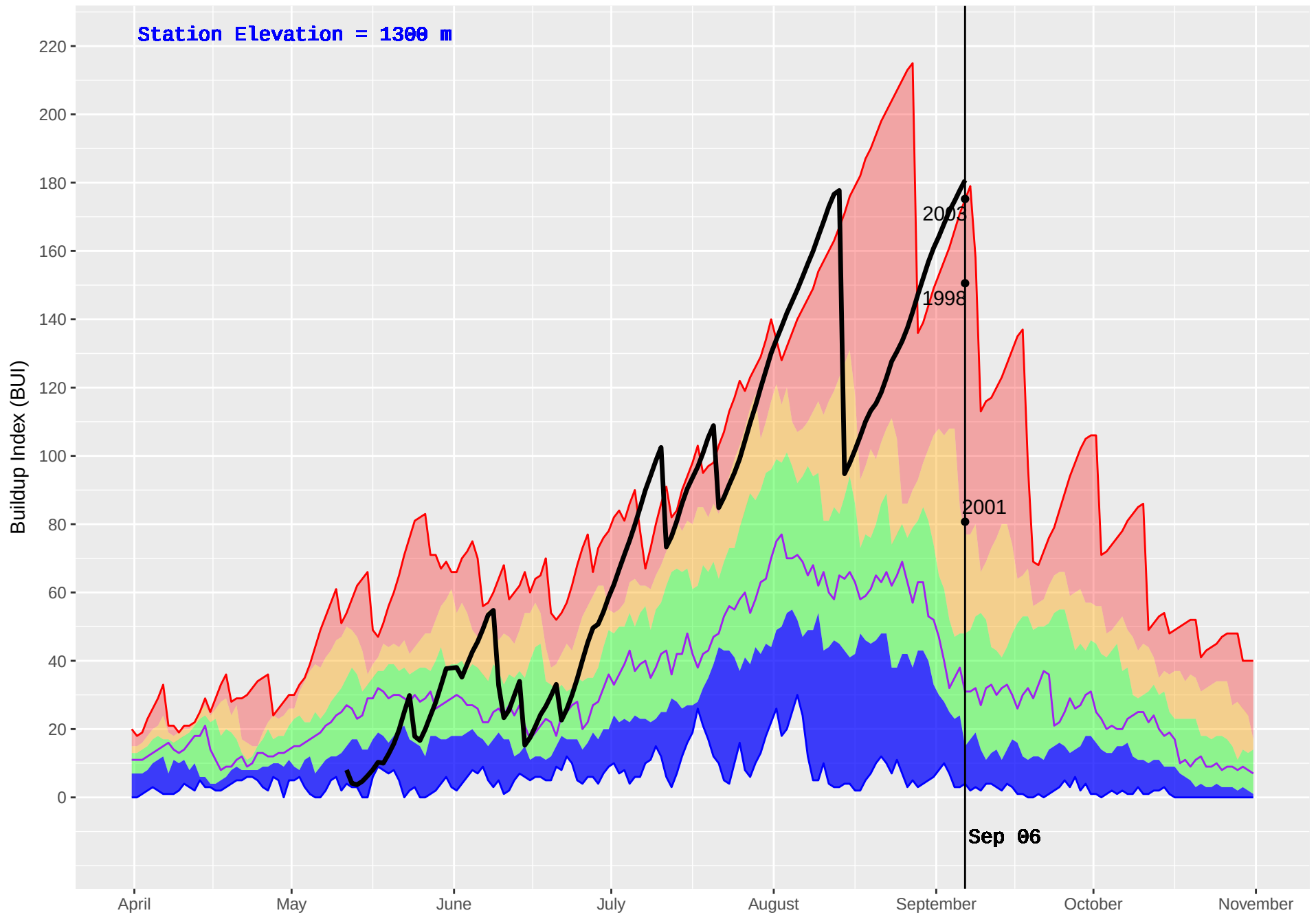
MARION (367) : Historical (1994–2016) and Current (2017) Noon Buildup Index (BUI)
