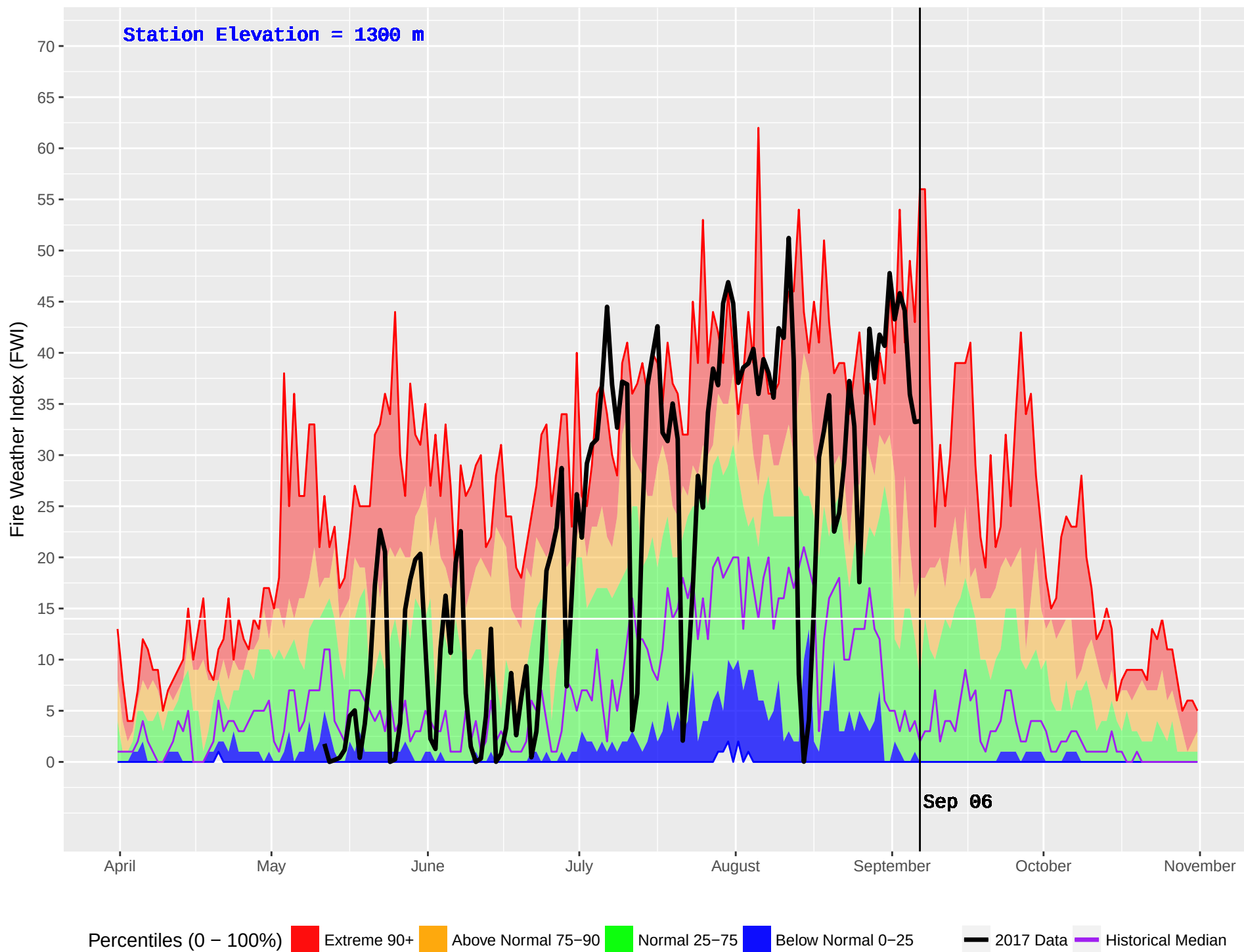
MARION (367) : Historical (1994–2016) and Current (2017) Noon Fire Weather Index (FWI)
